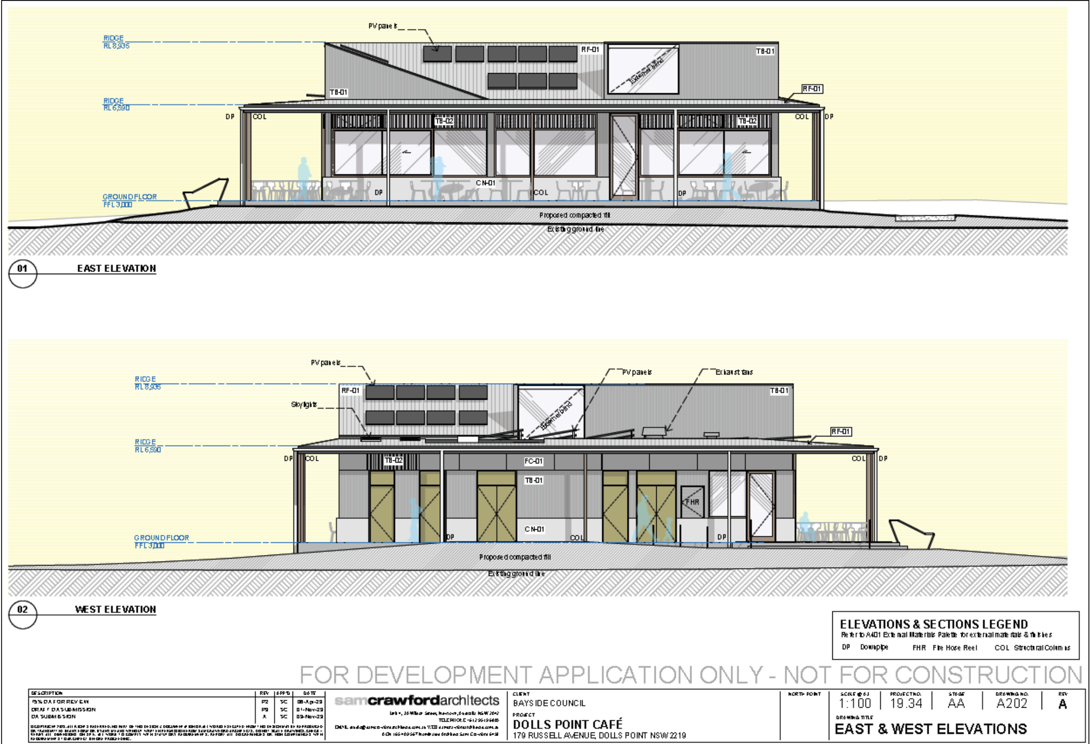
Item 1.1.4: Elevation Sections
