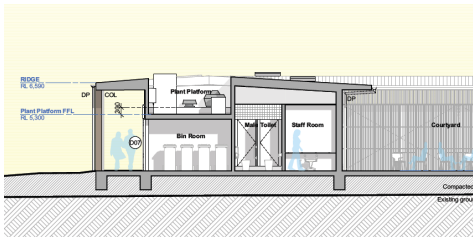
Figure 6b: Architectural section showing recessed open air plant platform at roof levelw planting
