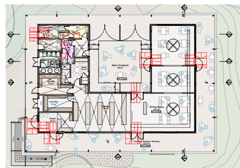
Figure 4e: Floor plan of proposed building.
