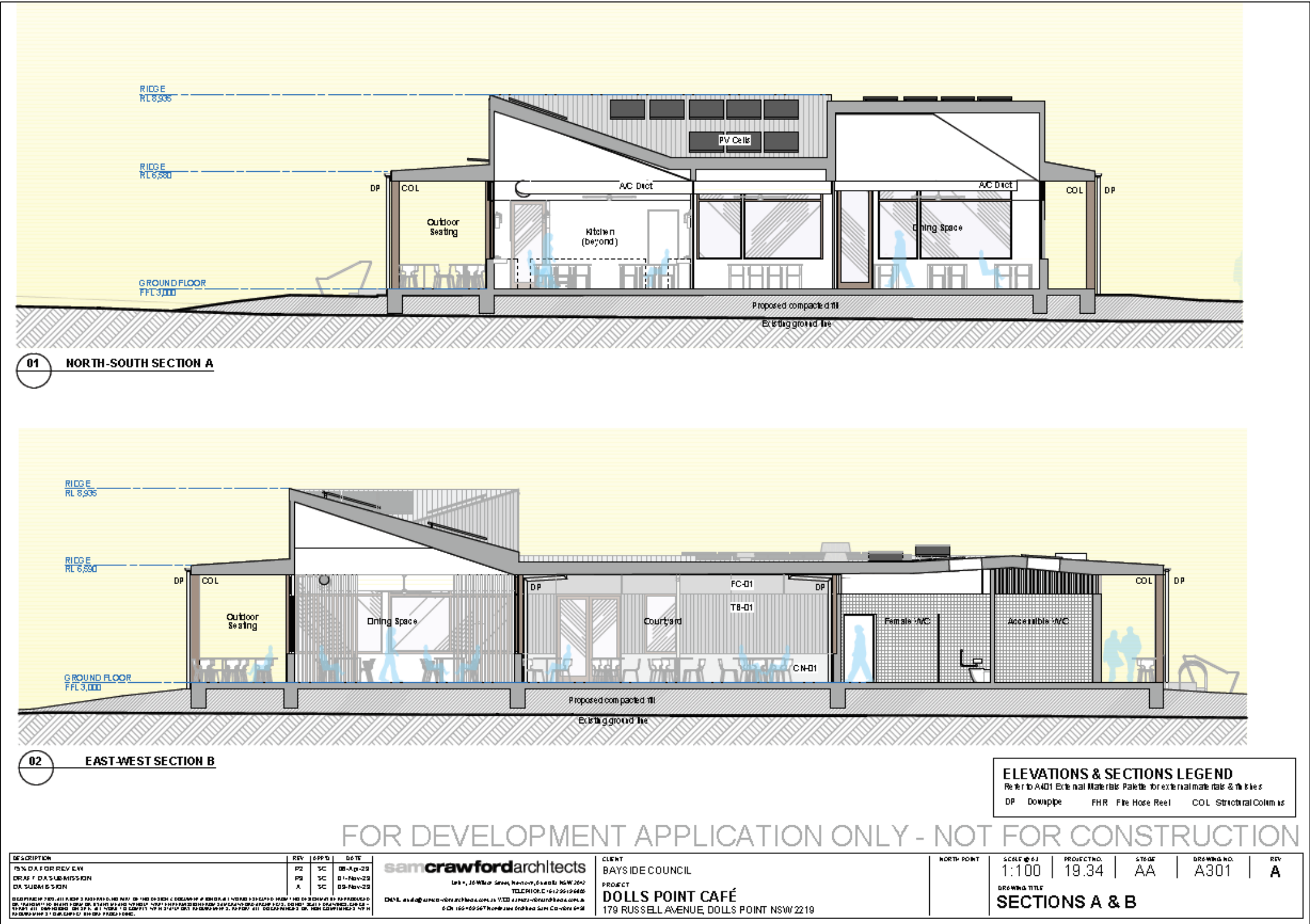
Item 1.1.5: Elevation Section
